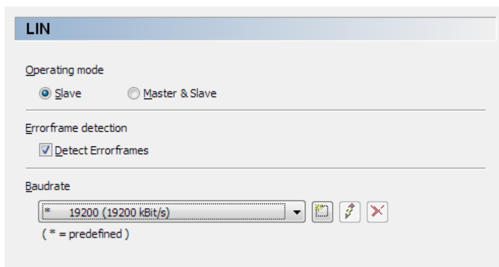
Figure 2.13: LIN Settings
