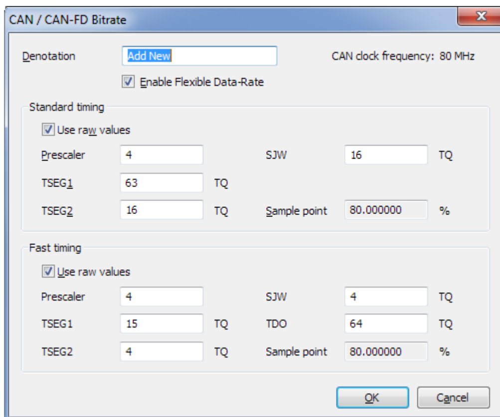
Figure 2.12: The CAN-FD bitrate dialog
